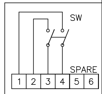
WIRING DIAGRAM
